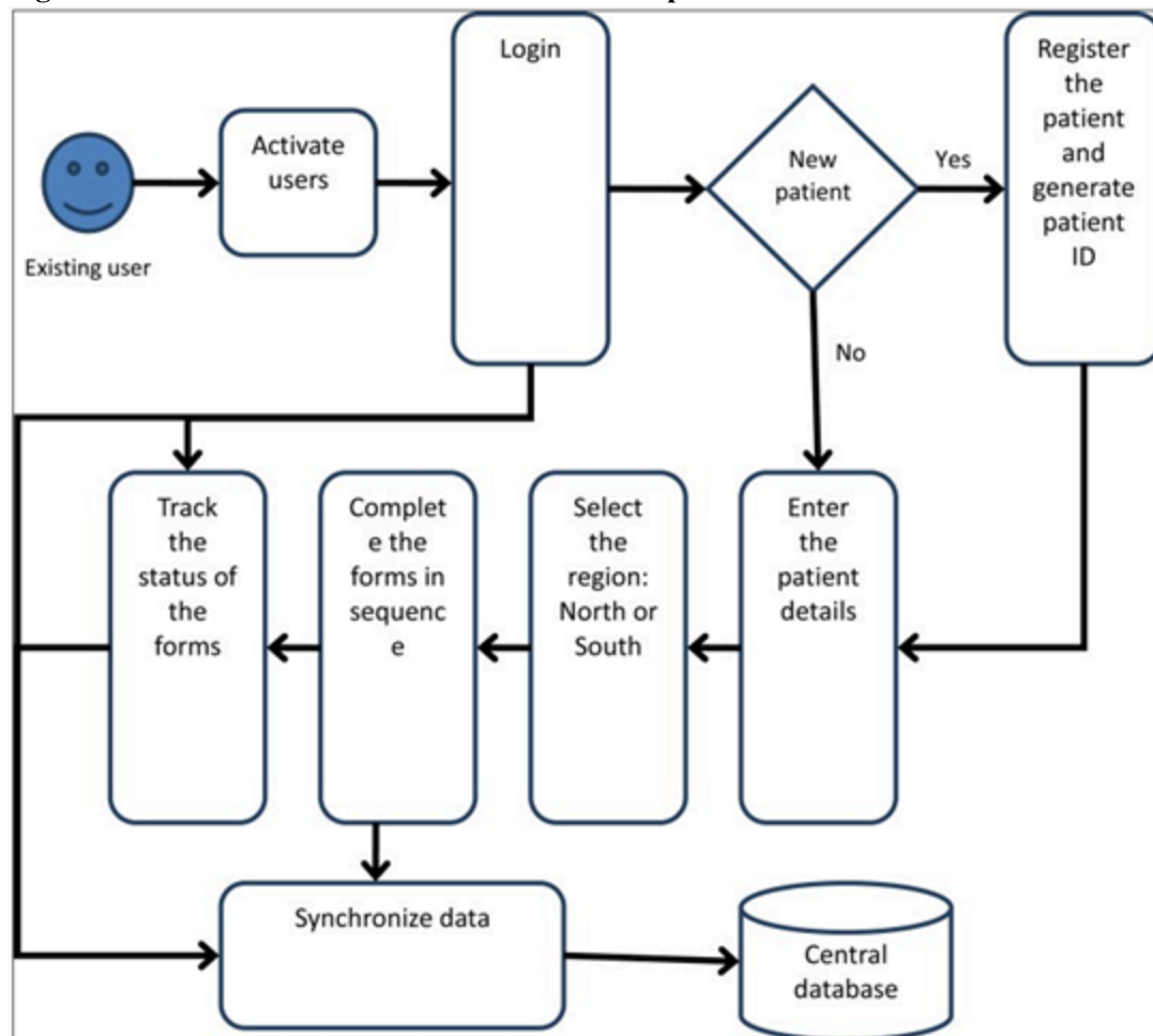
Figure 3: Data Flow for the Stand-alone Desktop-enabled Interactive Surveillance System
