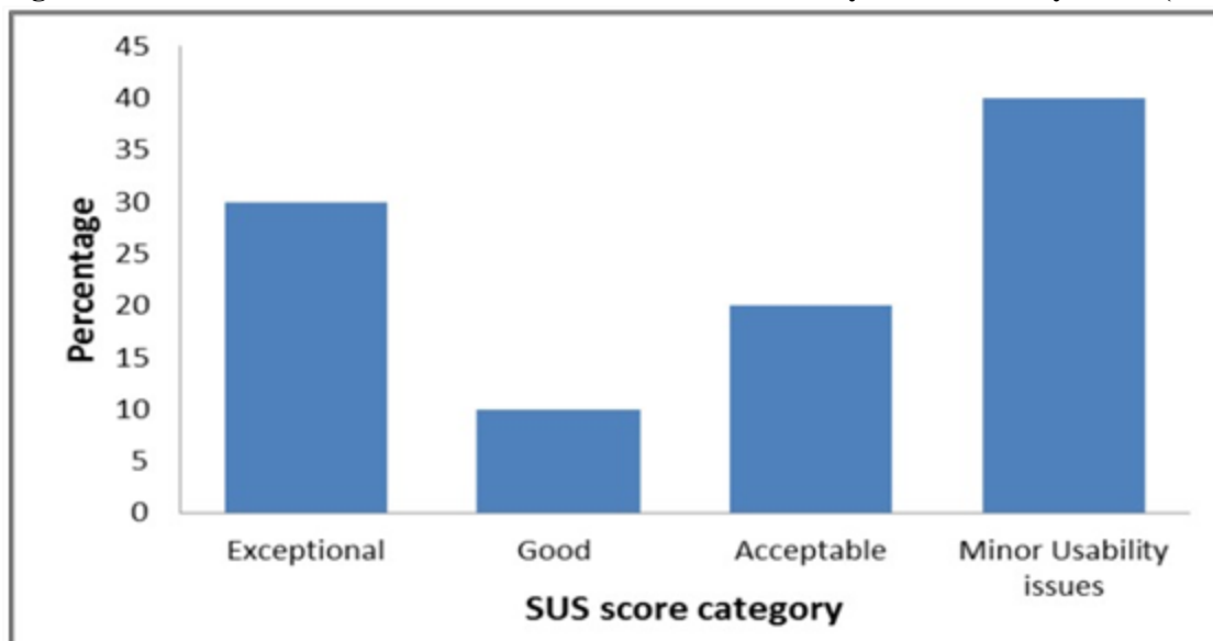
Figure 10: Percent Distribution of Individuals in the Four System Usability Scale (SUS) Score Categories
