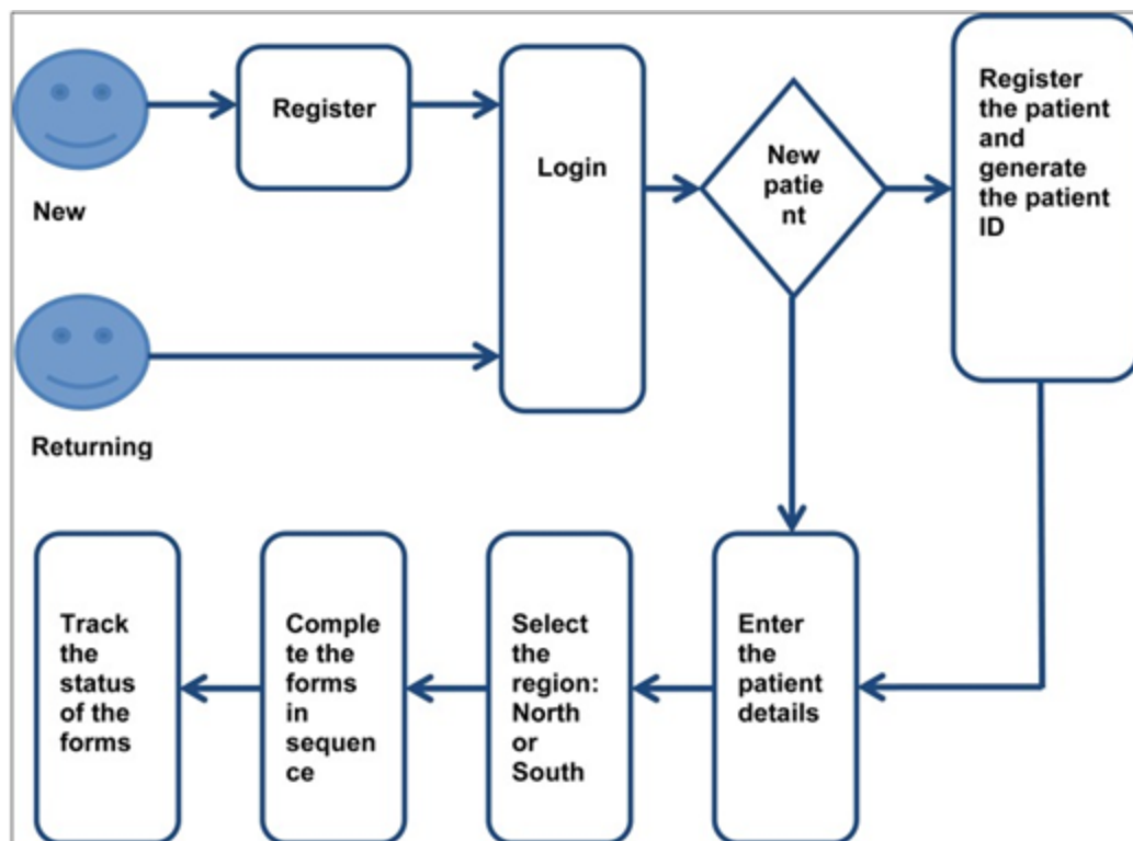
Figure 3: Data Flow for the Stand-alone Desktop-enabled Interactive Surveillance System
